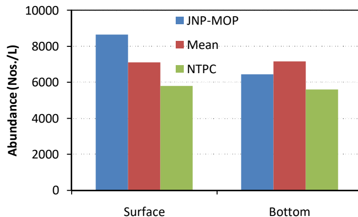
Fig. 7.2a: Comparison of phytoplankton abundance (No./L) at marine outfall points of JN Pharmacy Ltd. (JNP-MOP) and NTPC Ltd. with that of the mean phytoplankton abundance in surrounding stations of this zone during pre monsoon season
