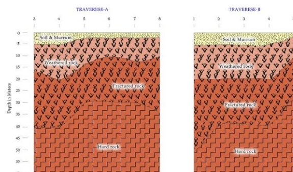
Fig. 7.3a: Vertical Lithological cross sections along Traverses- A and B
