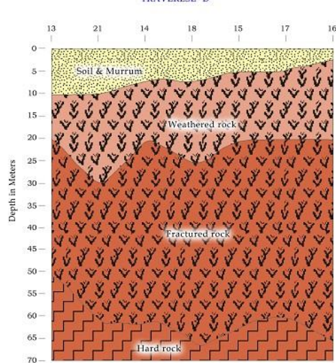
Fig. 7.3c: Ver. Cross section- Traverse- D
